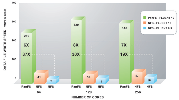
ACTIVESTOR STORAGE WITH THE PANFS PARALLEL FILE SYSTEM CONSISTENTLY OUTPERFORMS NFS BY 6X – 37X WHEN RUNNING FLUENT SOFTWARE
